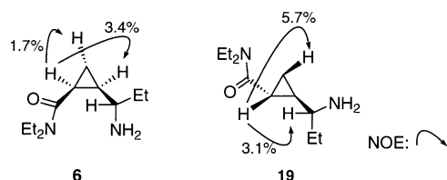
Figure 5. Determinations of stereochemistry of 6 and 19 .
