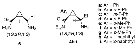
Figure 3. Derivatives of the PPDC modified at the 1-aromatic moiety.
