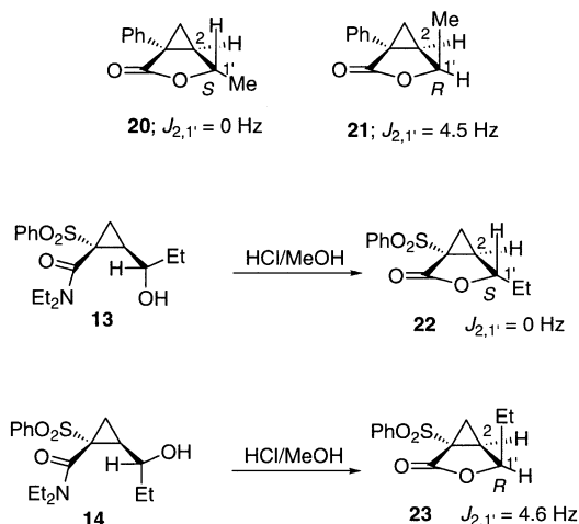
Figure 4. Determinations of the 1'-configurations of 13 and 14 .
