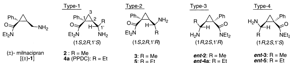
Figure 1. Milnacipran and its conformationally restricted analogues.
