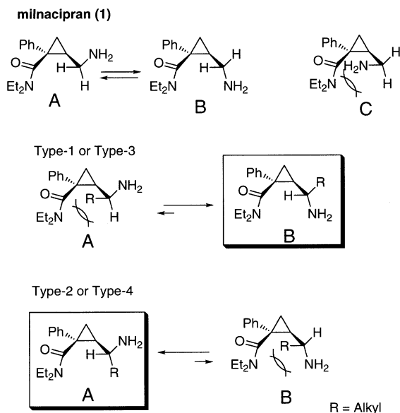
Figure 2. Conformational restriction of milnacipran by introducing an alkyl substituent at the 1'-position.
